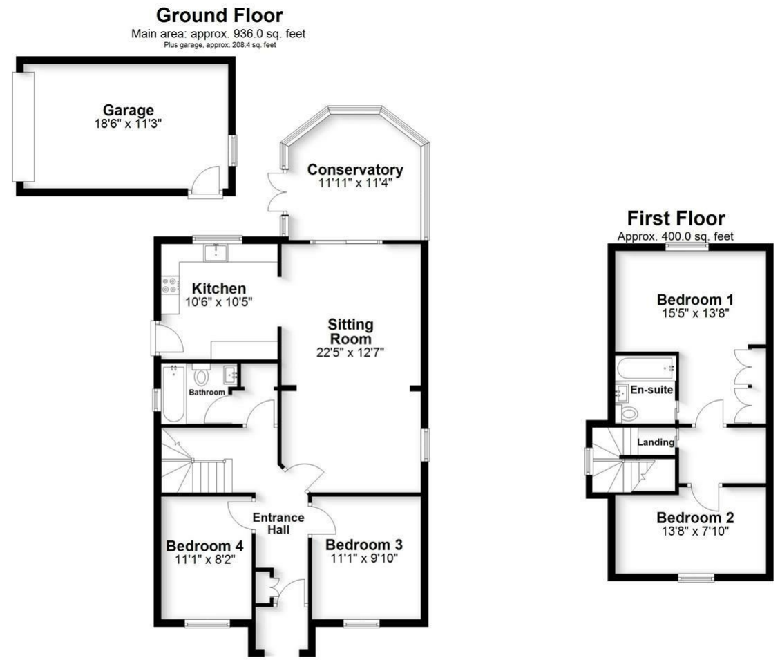
Ground Floor Main area: approx. 936.0 sq. feet Plus garage, approx. 208.4 sq. feet First Floor Approx. 400.0 sq. feet Main area: Approx. 124.1 sq. metres (1336.0 sq. feet) Plus garage, approx. 19.4 sq. metres (208.4 sq. feet) Produced for Cassidy & Tate Estate Agents. For guidance purposes, not to scale. Plan produced using PlanUp.
